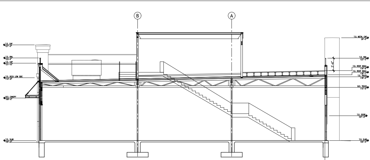
BUILDING SECTION 1/8"=1'-0" 1
