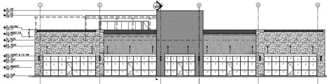
EAST ELEVATION 1/8"=1'-0" 1
